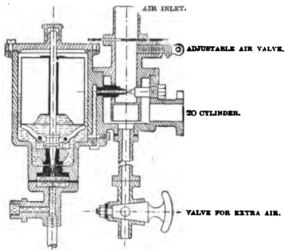
FIG. 814. —The Peugeot Carburetter. This has many points in common with other carburetters, except that the valve levers are differently arranged; the spraying nozzle at the side of the mixing tube, and the air-inlet from above.
